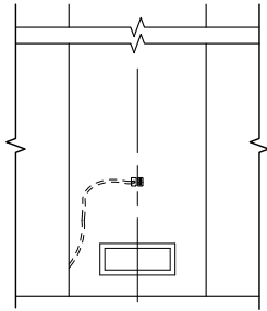
42" Contemporary Gas Fire Place
